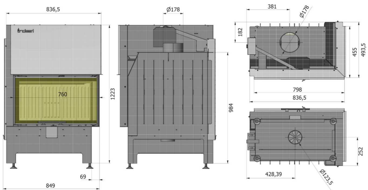
Abb. 2.13. Heatro 69PH
